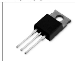
P-TO220-3-1.
