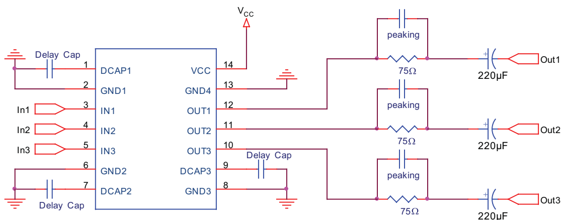
Figure 15. Schematic
