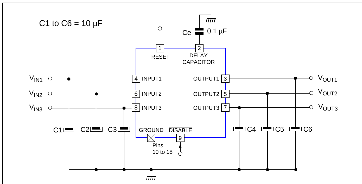
Figure 6: STV8162D Typical Application
