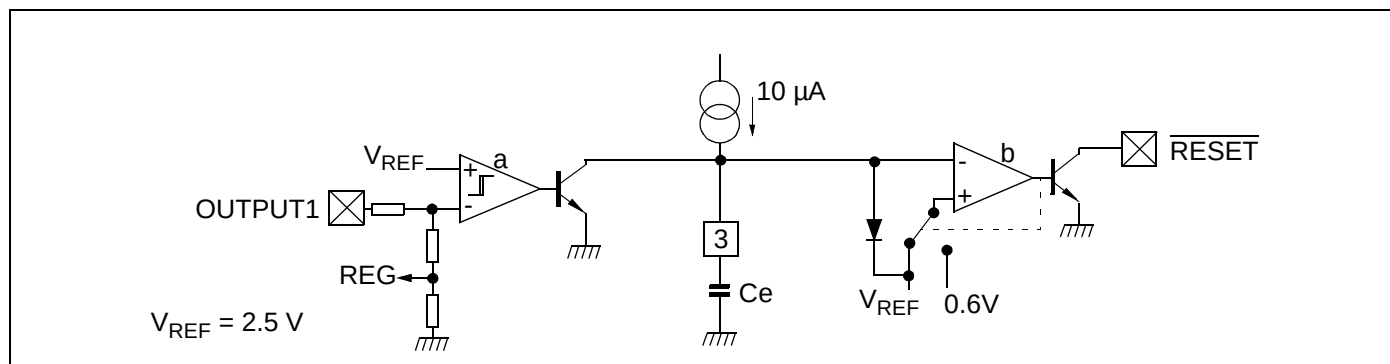
Figure 3: Reset Diagram
