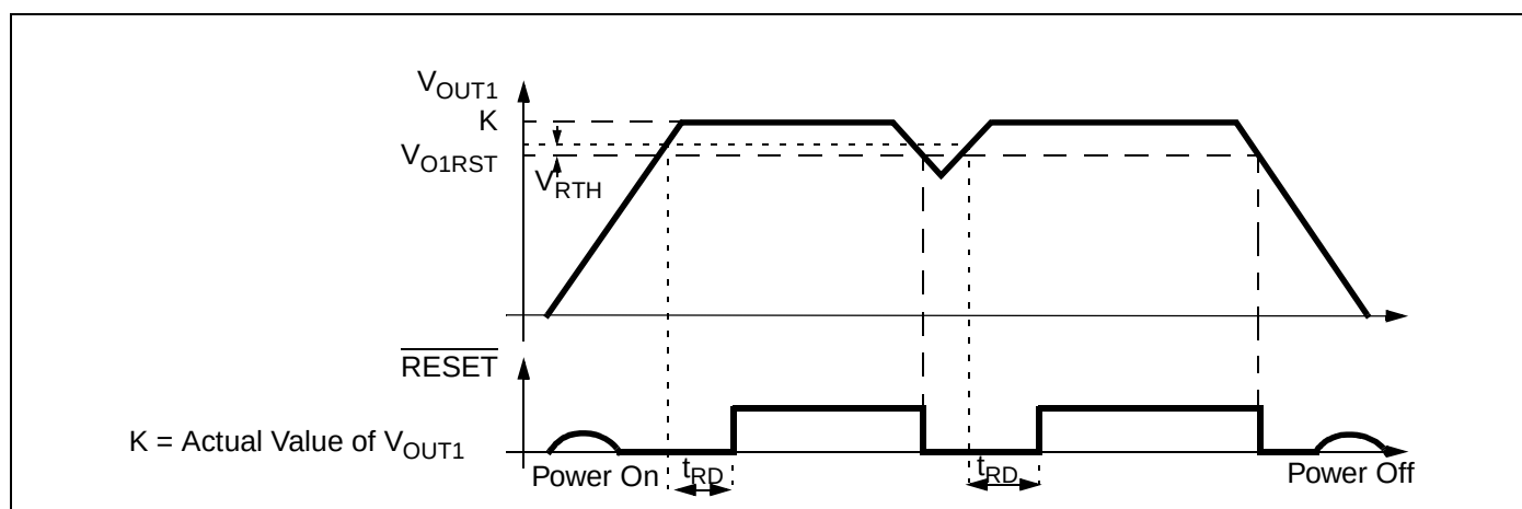
Figure 4: Internal Reset Voltage
