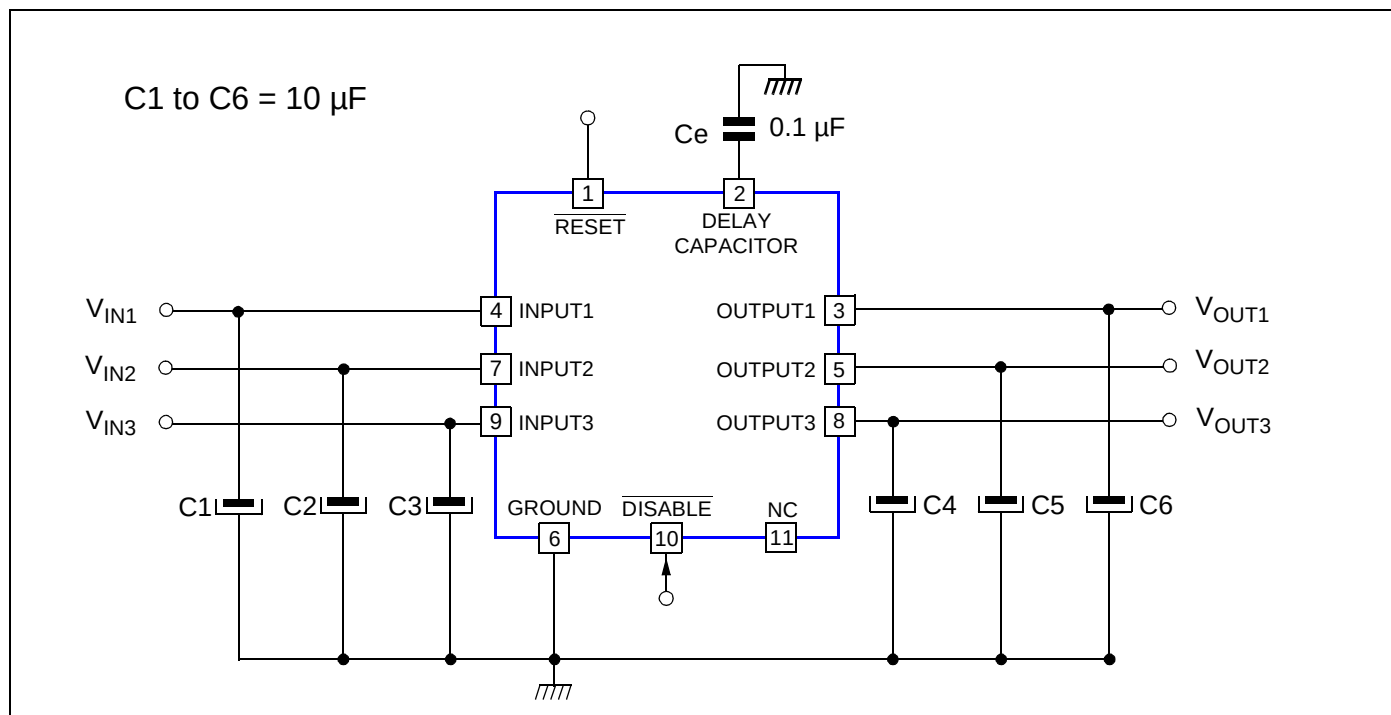
Figure 5: STV8162 Typical Application
