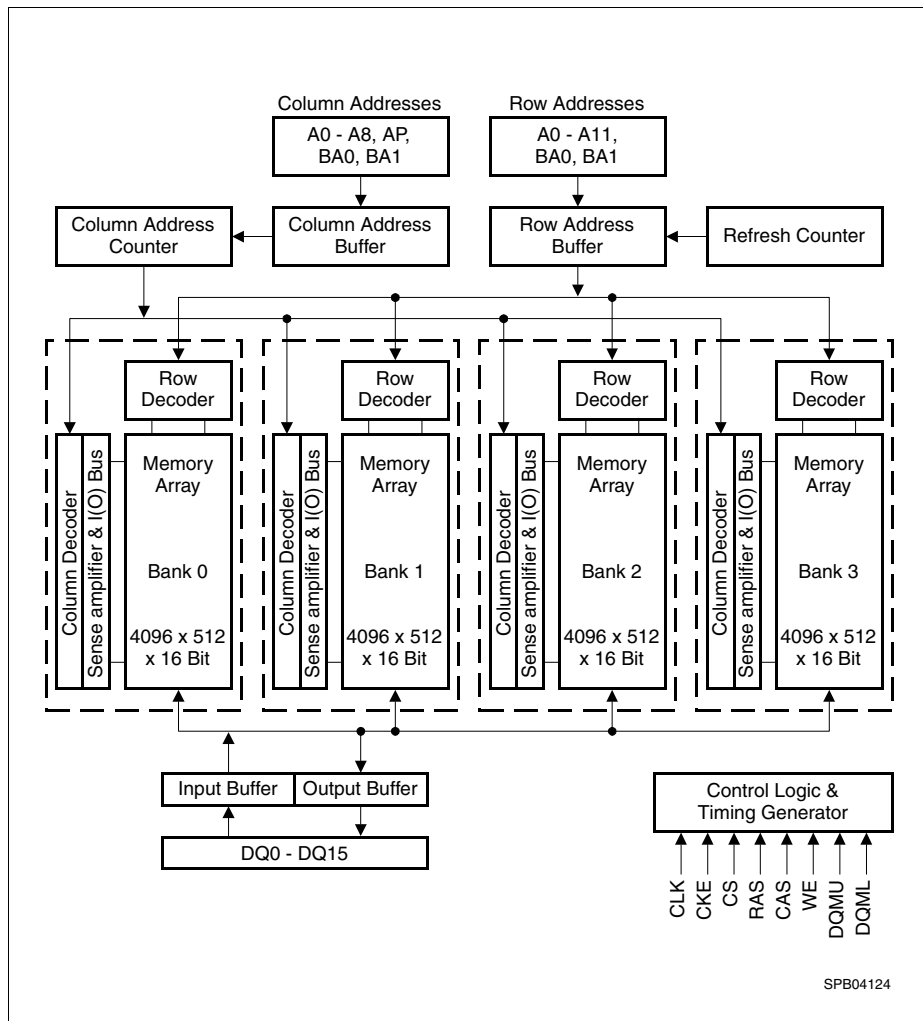
Block Diagram: 8Mb x16 SDRAM (12 / 9 / 2 addressing)
