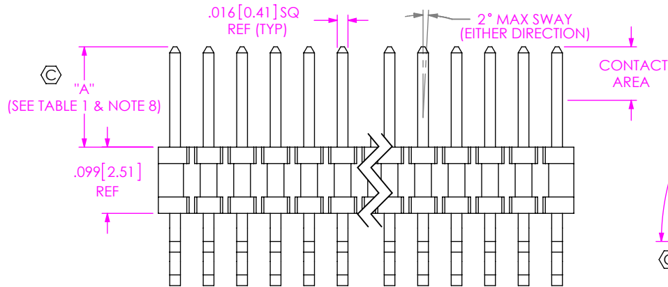
FIG 1 FTSH-1XX-XX-XXX-D-RA SHOWN
