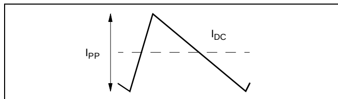
Figure 2: Vertical Amplitude and Position
