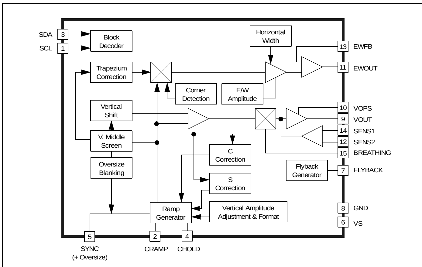
Figure 1: STV9306B Block Diagram
