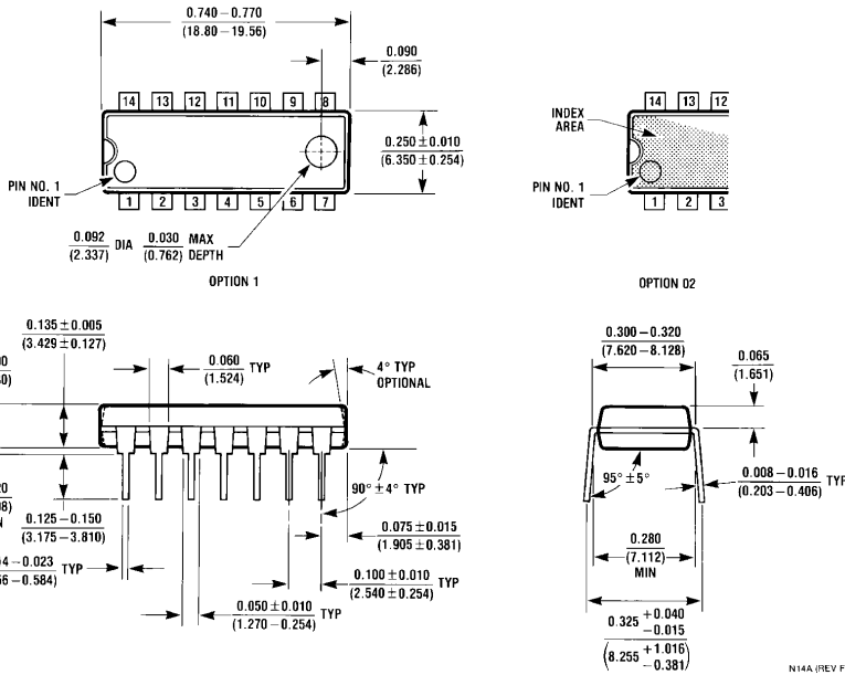
Molded Dual-In-Line Package (N) Order Number LM319AN or LM319N NS Package Number N14A
