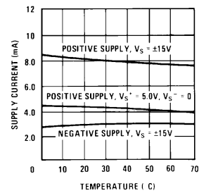
Supply Currents
