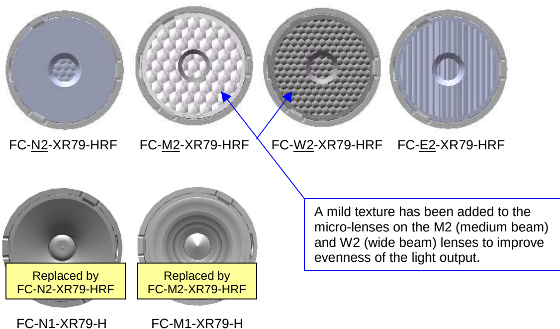
Figure 1. Identifying the lenses by their front views
