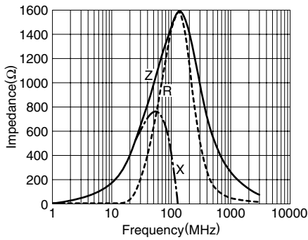
MMZ1608D100C
