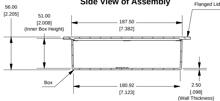
SECTION B-B Side View of Assembly
