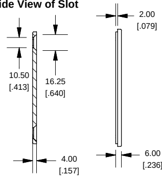
SECTION C-C Side View of Slot
