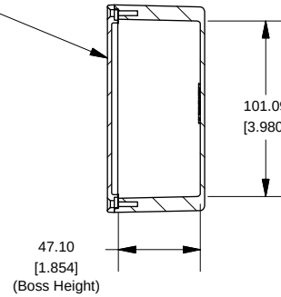
SECTION A-A End View of Assembly
