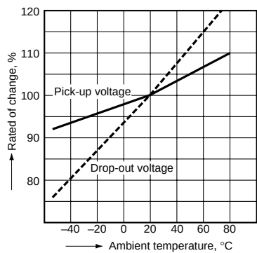
5. Rate of change of pick-up and drop-out voltage 2 Form C single side stable
