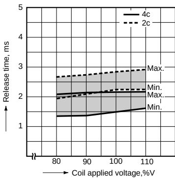
4. Release time for single side stable
