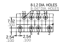
PC board pattern (Copper-side view)
