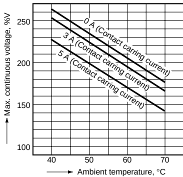
6.-(1) Ambient temperature vs Max. continuous voltage Sample: NC2D-P-DC24 V (2c slim single side stable)
