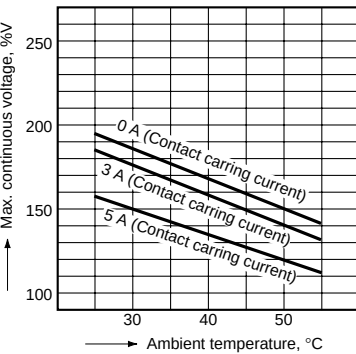
6.-(2) Ambient temperature vs Max. continuous voltage Sample: NC2D-P-DC110 V (2c slim single side stable), NC4D-P-DC24 V (4c slim single side stable)
