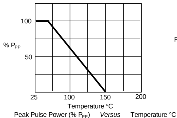
Figure 2 - Derating Curve
