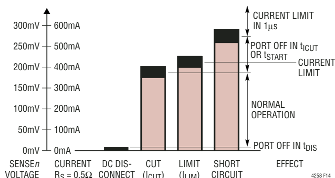
Figure 16. LTC4258 Current Sense and Limits
