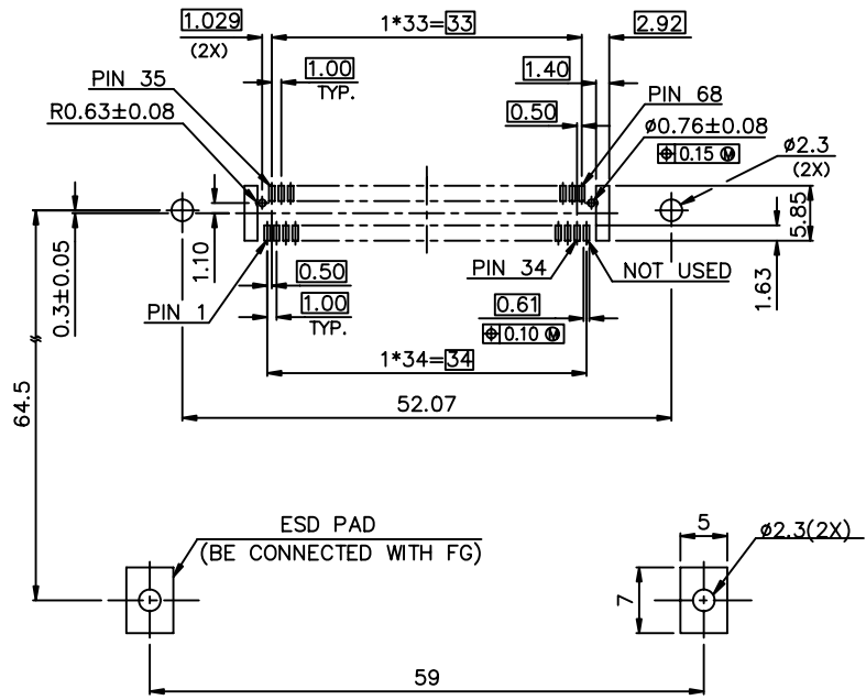
FOR 10003526-0XX(M)CALF/1XX(M)CALF P.C.B LAYOUT BOARD VIEW FROM CONNECTOR MOUNTED SIDE
