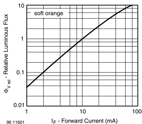
Fig. 12 - Relative Luminous Flux vs. Forward Current
