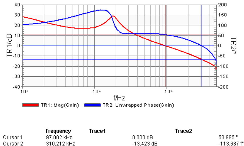
Figure 41: CH2 Bode Plot with 6A load, CH1 disabled. F_o = 97 \text{ kHz} , Phase Margin = 54 Degrees
