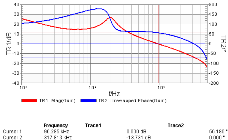
Figure 40: CH1 Bode Plot with 6A load, CH2 disabled. F_o = 96.3 \text{ kHz} , Phase Margin = 56.2 Degrees
