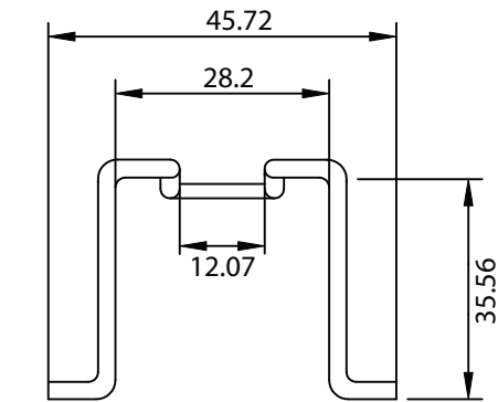
CLIP 1.82mm Dia. Stainless Steel Wire
