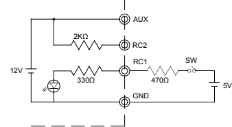
Using external voltage
