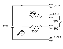
Using internal 12V auxiliary output
