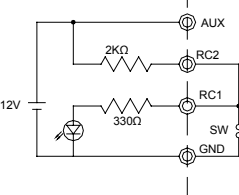
Using internal 12V auxiliary output
