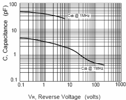
Figure 2. Capacitance
