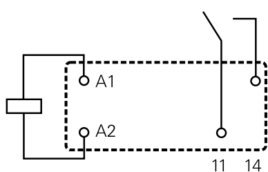
1 form A (NO) contact
