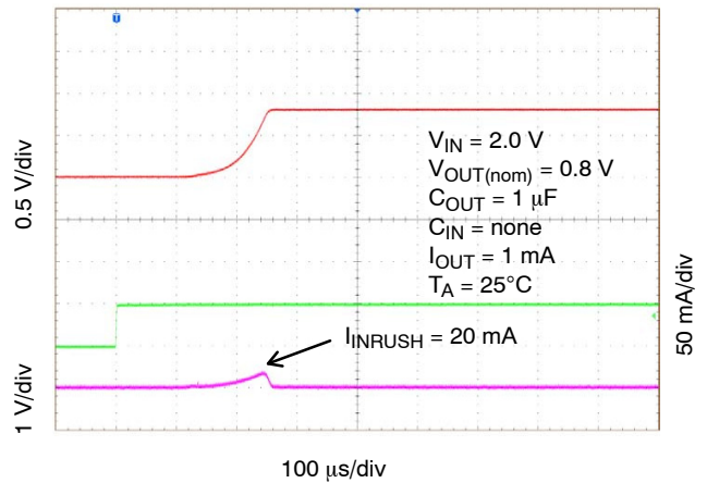
Figure 38. Enable Turn-On Response, V_{OUT} = 0.8 V, C_{OUT} = 1 μF
