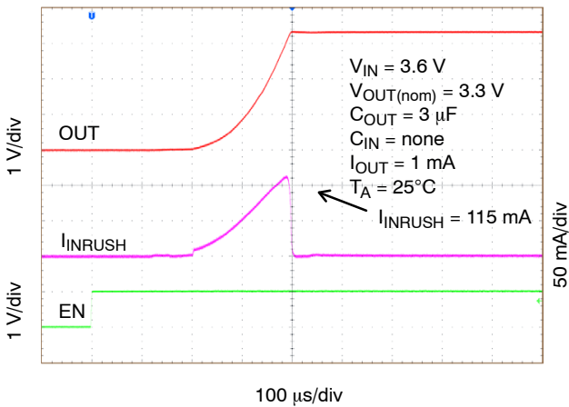
Figure 37. Enable Turn-On Response, V_{OUT} = 3.3 V, C_{OUT} = 3 μF
