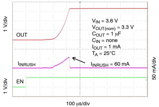
Figure 36. Enable Turn-On Response, V_{OUT} = 3.3 V, C_{OUT} = 1 μF
