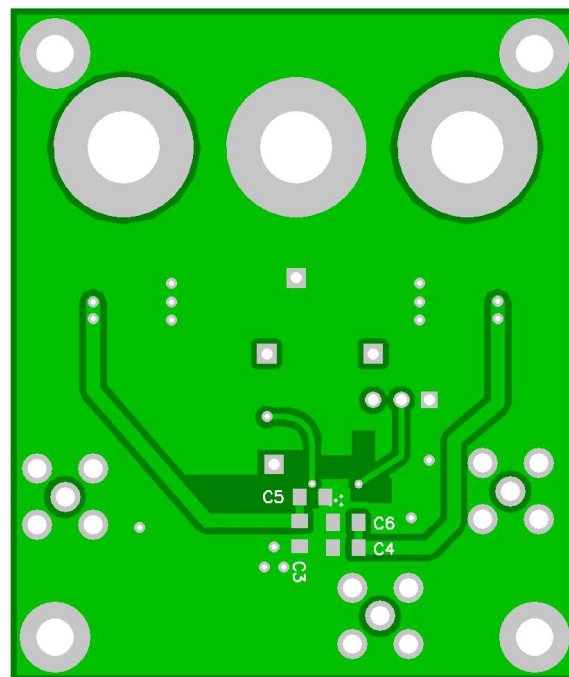
Figure 64. THS3120 EVM Board Layout (Bottom Layer)
