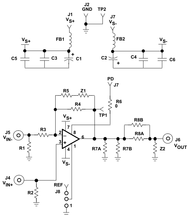
Figure 62. THS3120 EVM Circuit Configuration
