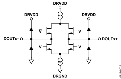
Figure 35. Equivalent Digital Output Circuit
