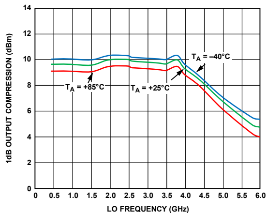
Figure 5. SSB Output 1dB Compression Point ( \text{OP1dB} ) vs. LO Frequency ( f_{\text{LO}} ) and Temperature
