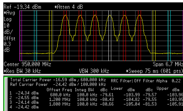
Figure 69. ADL5375-05 GSM/EDGE(8-PSK) 6 Carriers Adjacent and Alternate Channel Power Performance at 950 MHz; Output Power(1 Carrier/100 KHz) = -24.4 dBm LO Drive = 0 dBm
