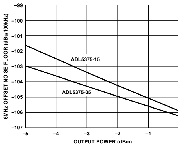
Figure 70. GSM/Edge (8-PSK) 6 MHz Offset Noise at 940 MHz vs. Output Power, LO Drive = 0 dBm
