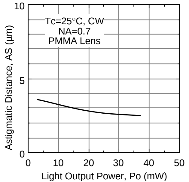
Astigmatic Distance
