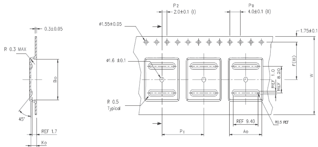
Figure 26. TQFP-64 power lead-less tape and reel shipment (suffix "TR") (part 1)
