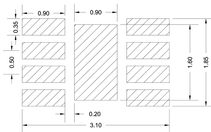
Figure 30. DFN8 2 x 2 wettable flank recommended footprint
