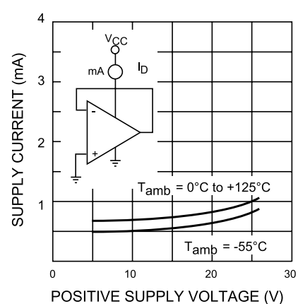
Figure 13. Supply current
