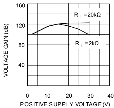
Figure 14. Voltage gain
