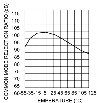
Figure 18. Common-mode rejection ratio
