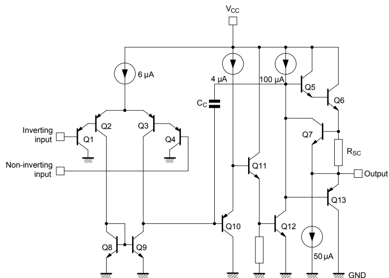
Figure 1. Schematic diagram (1/2 LM2904H/AH)
