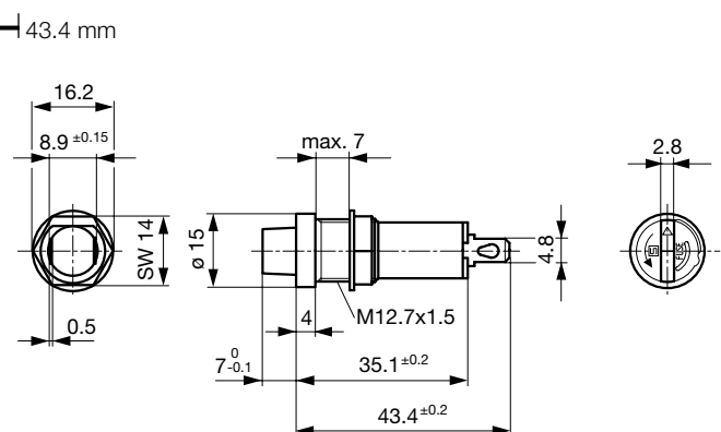
Variant Fingergrip 0031.3911
