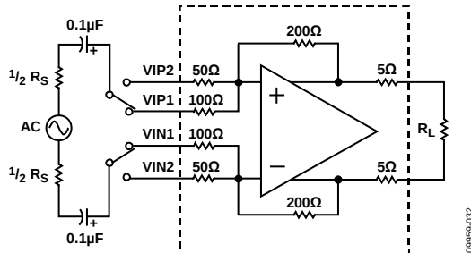
Figure 30. Basic Structure
