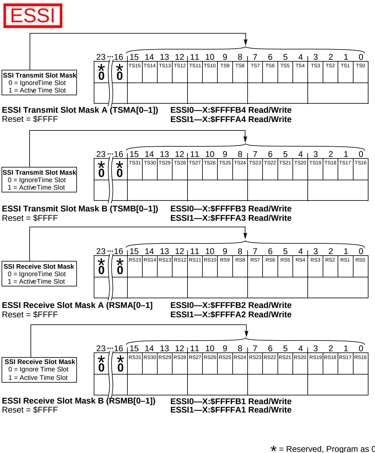
Figure B-17. ESSI Transmit and Receive Slot Mask Registers (TSM, RSM)
