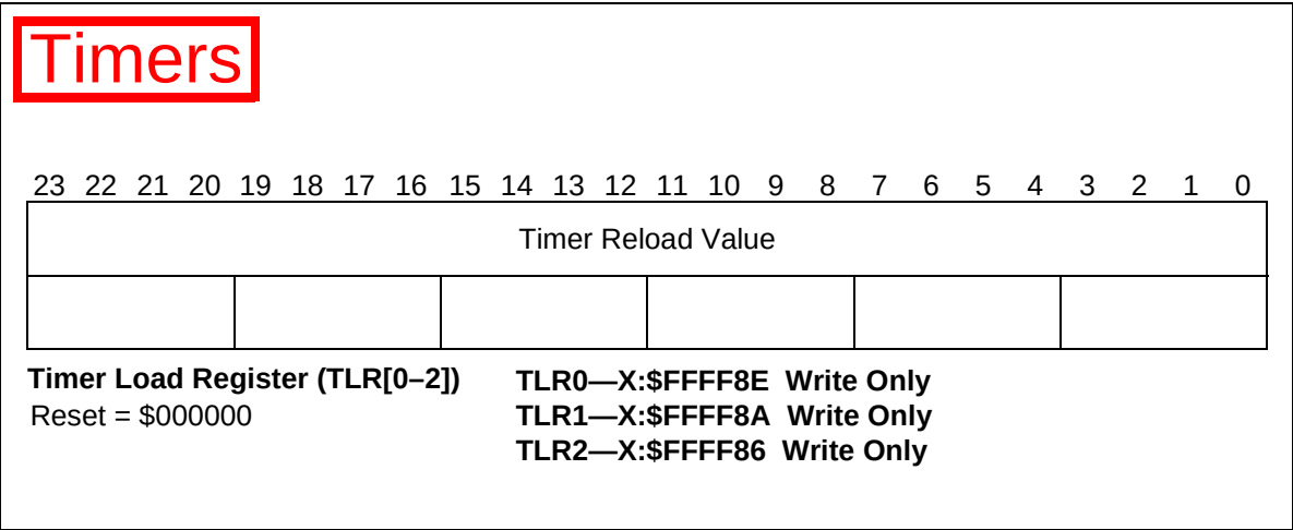
Figure B-22. Timer Load Registers (TLR)
