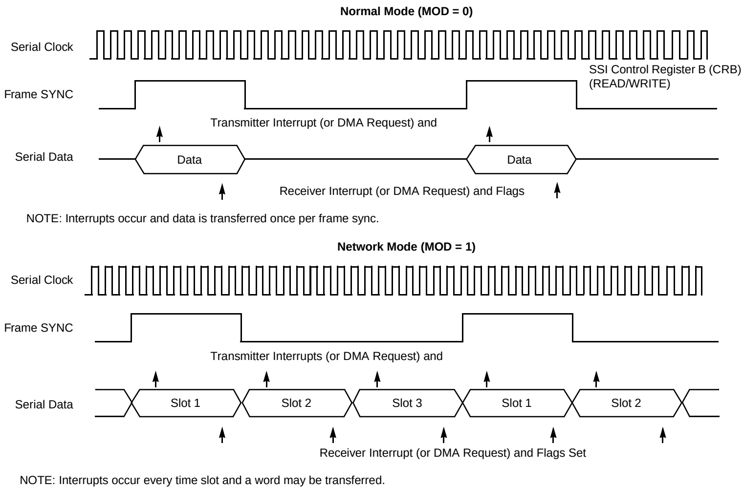
Figure 7-8. CRB MOD Bit Operation
