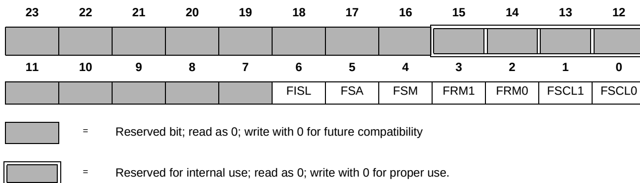
Figure 10-13. EFCOP ALU Control Register (FACR)
