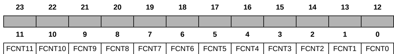
Figure 10-11. Filter Count (FCNT) Register
