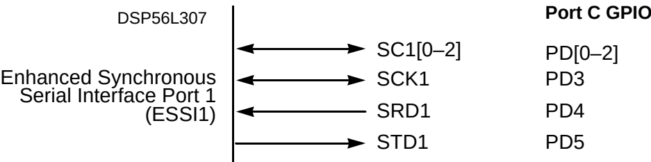
Figure 5-4. Port D Signals
