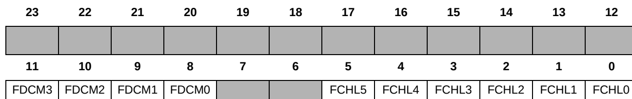
Figure 10-14. Decimation/Channel Count Register (FDCH)
