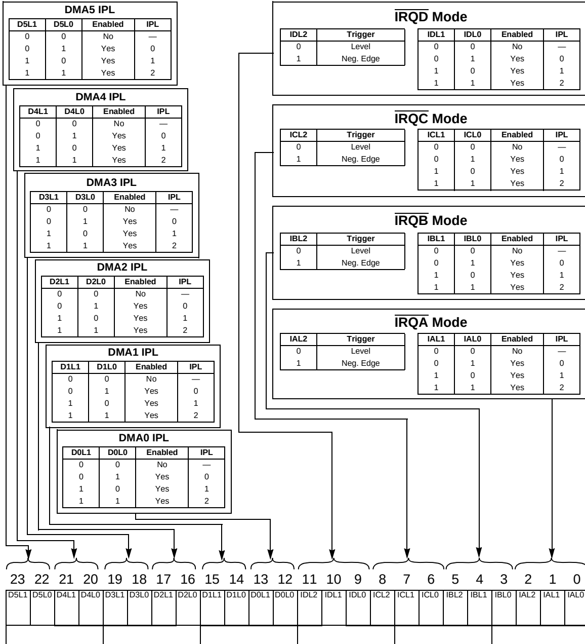
Figure B-3. Interrupt Priority Register-Core (IPRC)
