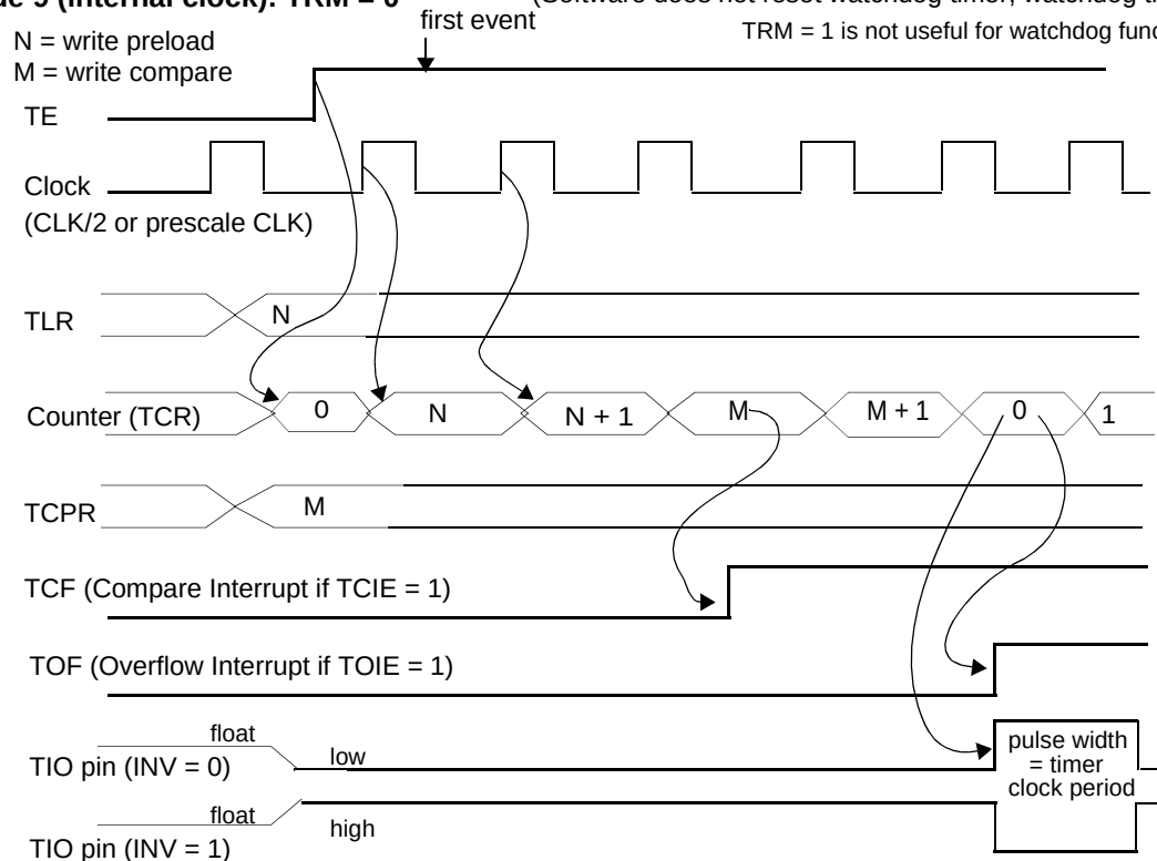
Figure 9-18. Watchdog Pulse Mode
