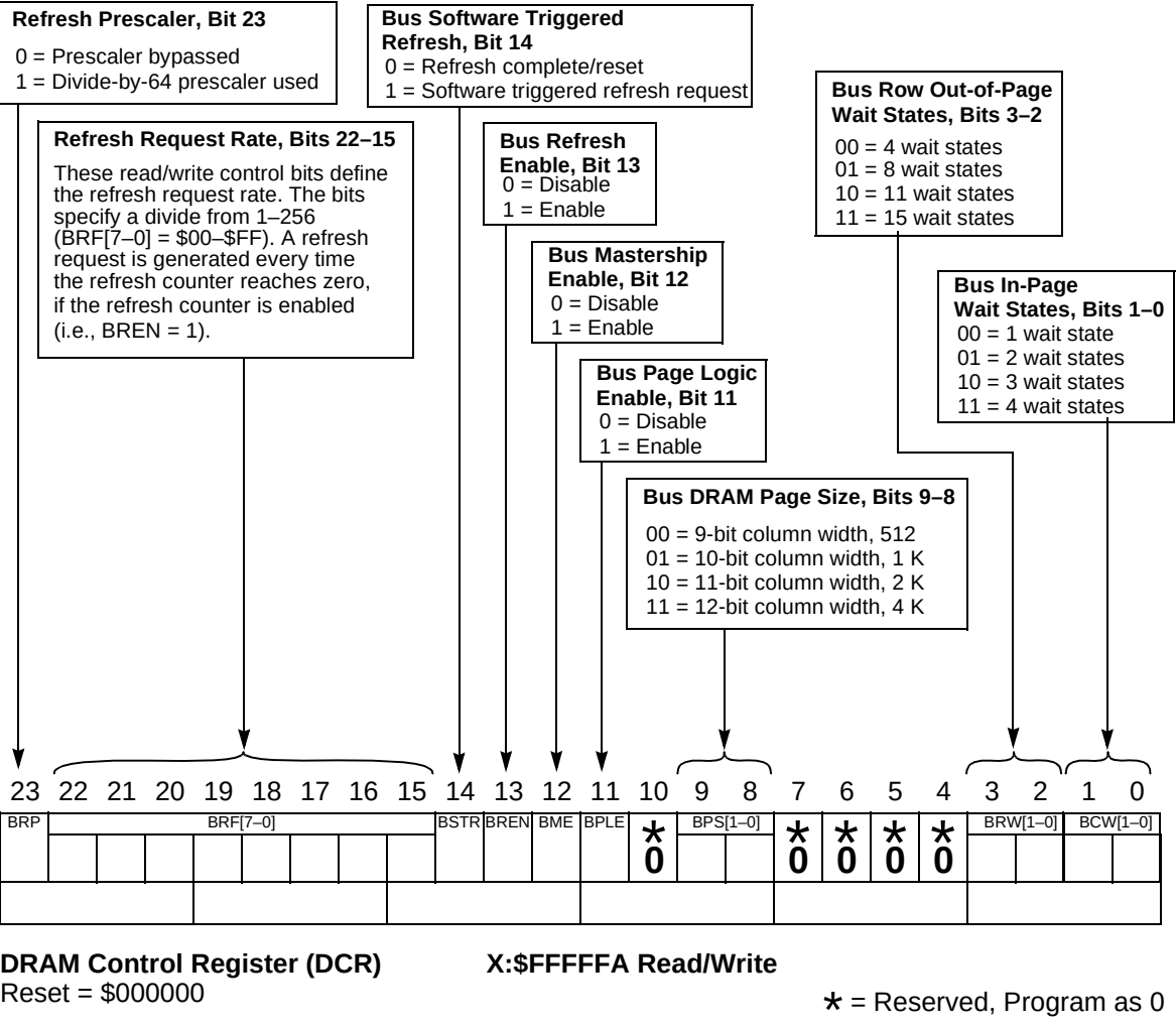
Figure B-7. DRAM Control Register (DCR)
