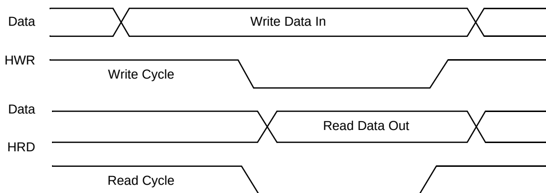
Figure 6-13. Single-Strobe Mode
