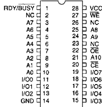
CERDIP, PDIP, SOIC Top View
