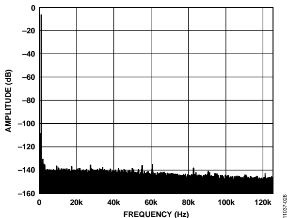
Figure 18. 1 kHz Input Tone, -6 dBFS Input FFT (AVDD1 = 5 V, AVDD2 = 5 V, IOVDD = 3.3 V, V_{REF} = 2.5 V, Output Data Rate = 250 kSPS)
