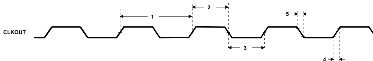
Figure 5-10. CLKOUT Timing
