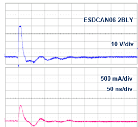
Figure 10. Response to ISO 7637-3 Pulse 3b : +150 V
