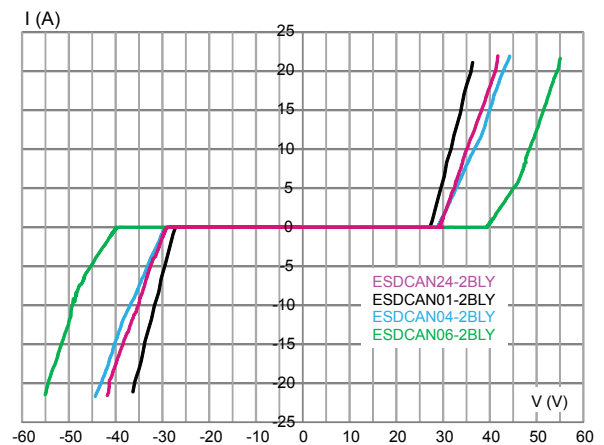
Figure 14. TLP
