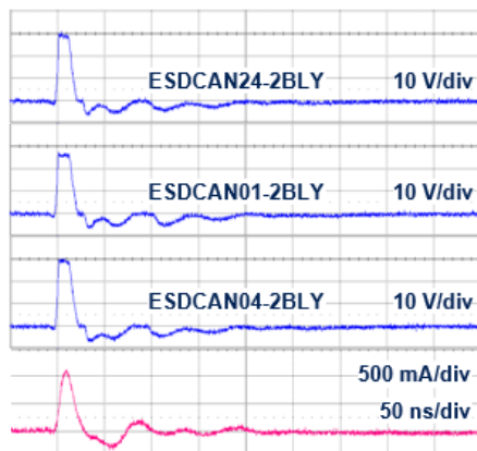
Figure 10. Response to ISO 7637-3 Pulse 3b : +150 V
