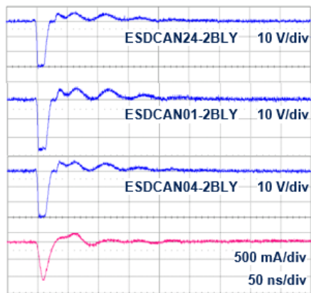
Figure 9. Response to ISO 7637-3 Pulse 3a: -150 V
