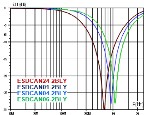
Figure 13. S21 attenuation
