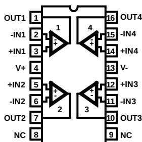
HA5104/5114 (SOIC) TOP VIEW
