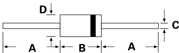
DO-204AC (DO-15)
