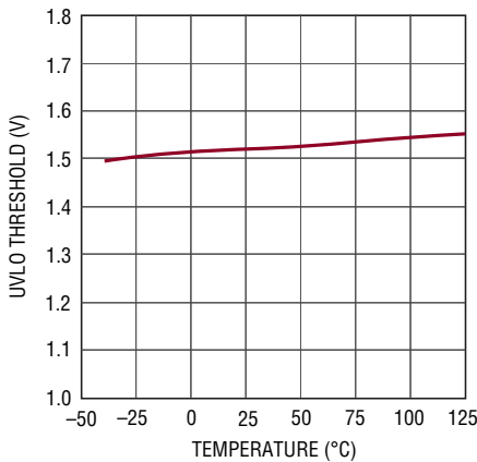
UVLO Threshold
