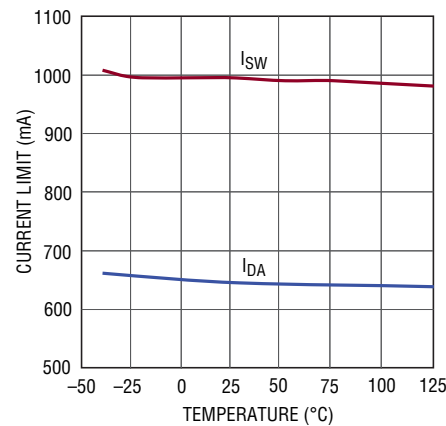
SW and DA Current Limit
