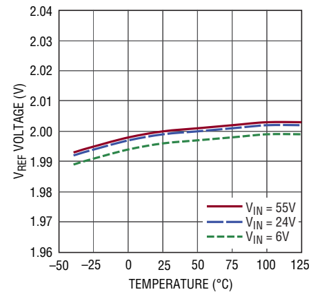
V_{REF} Voltage
