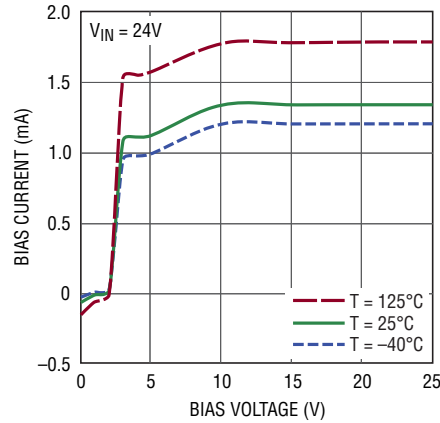
BIAS Quiescent Current
