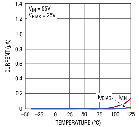
V_{IN} , BIAS Shutdown Current
