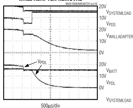
PDS-PDL SWITCHOVER, WALL ADAPTER REMOVAL
