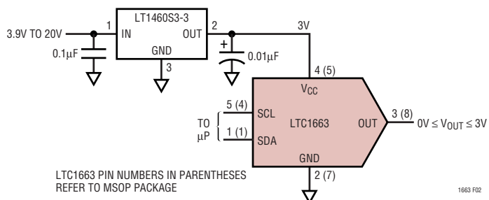
Figure 2. LT1460 As Power Supply for the LTC1663
