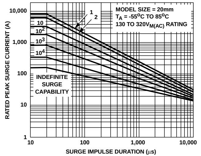
FIGURE 7. REPETITIVE SURGE CAPABILITY FOR V130LA20C TO V320LA40C
