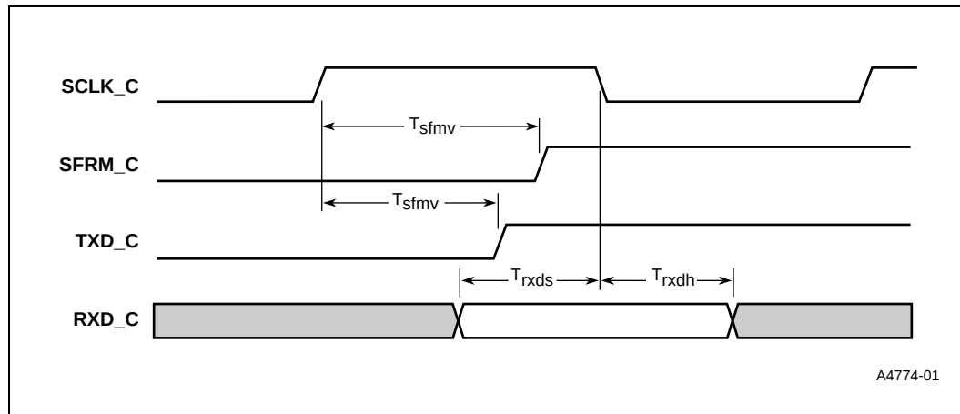
Figure 9. SSP AC Timing Definitions
