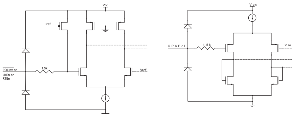
Figure 3-2: GN2014A Control Input Equivalent Circuits
