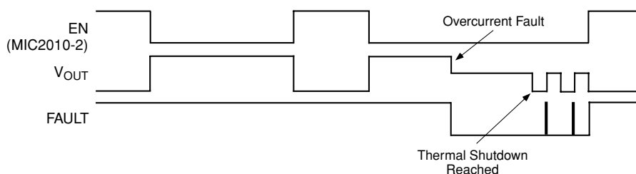
Figure 6. MIC2010 System Timing
