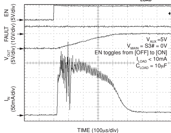
AUX Inrush Current into Small C_LOAD
