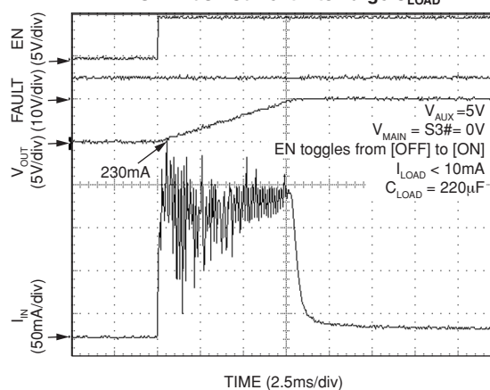
AUX Inrush Current into Large C_LOAD
