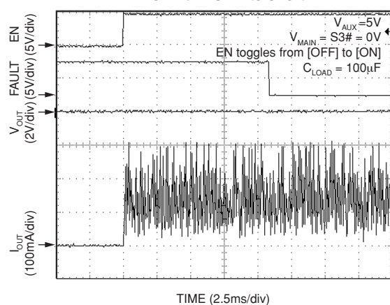
AUX Turn-On into Short
