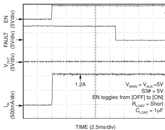
Main Turn-On into Short
