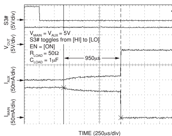
Main-to-AUX Cross Conduction
