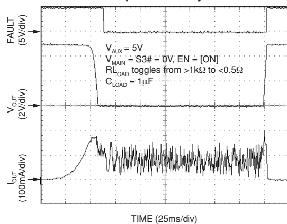
AUX Ramped to Short by MOSFET
