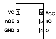
IDT8N3SV76 6-lead ceramic 5mm x 7mm x 1.5mm package body CD Package Top View
