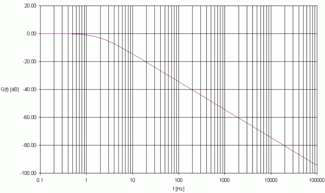
Figure 23 - Jitter Transfer Function
