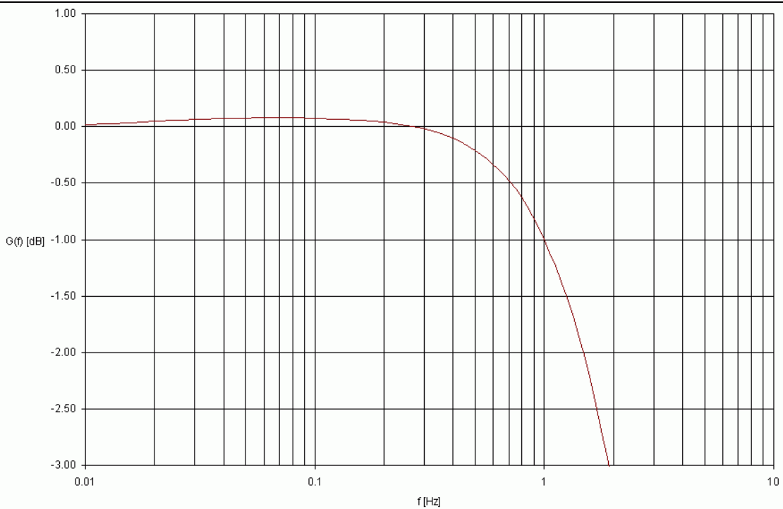
Figure 24 - Jitter Transfer Function - Detail
