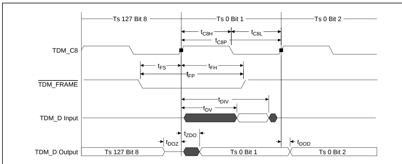
Figure 29 - H.110 Timing Diagram
