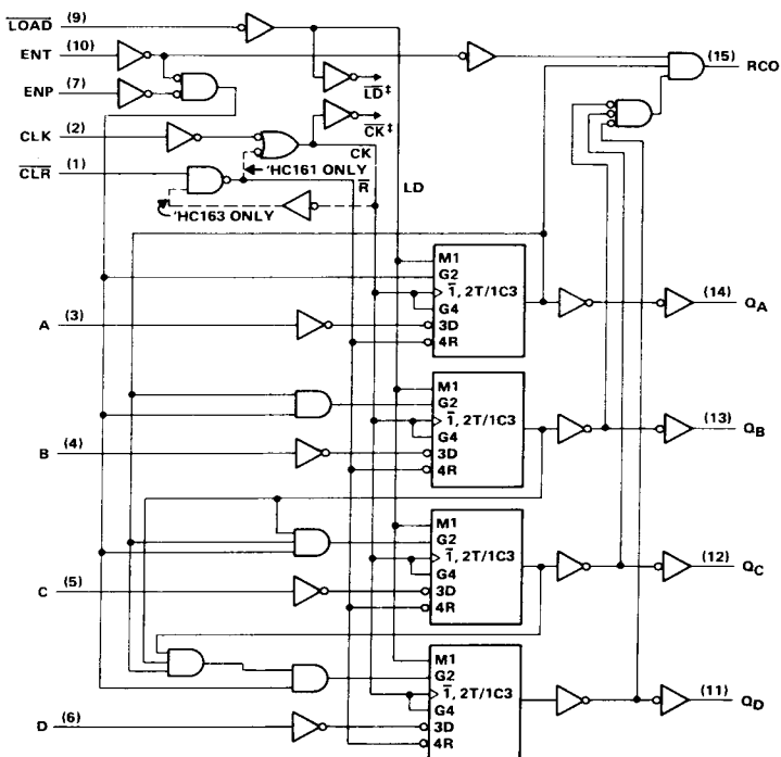
'HC161 and 'HC163 logic diagram (positive logic)
