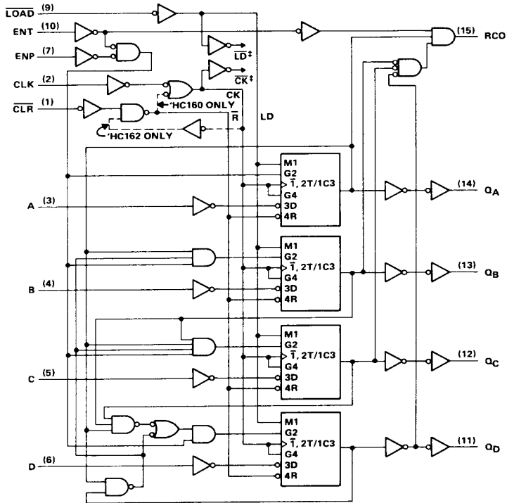
'HC160 and 'HC162 logic diagram (positive logic)
