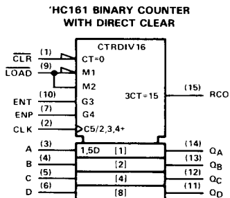
'HC161 and 'HC163 logic diagram (positive logic)
