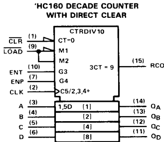
'HC160 and 'HC162 logic diagram (positive logic)
