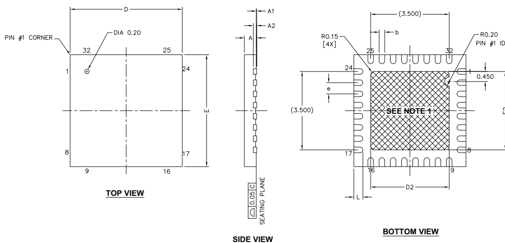
Figure 26. 32-pin QFN ( 5 \times 5 \times 0.55 mm) LQ32 3.5 \times 3.5 E-Pad (Sawn) Package Outline, 001-42168
