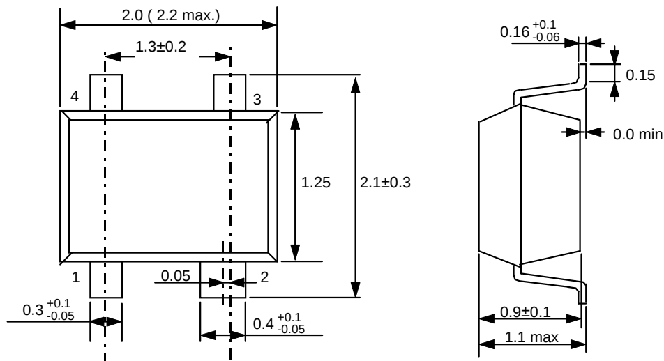
(1) SC-82AB
