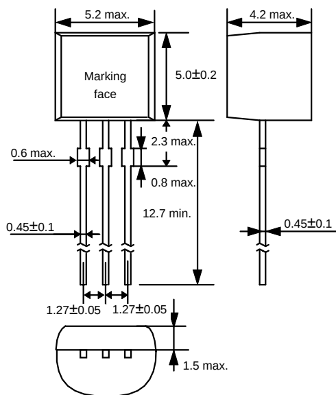
(2) TO-92
