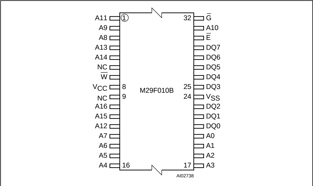
Figure 3. TSOP connections
