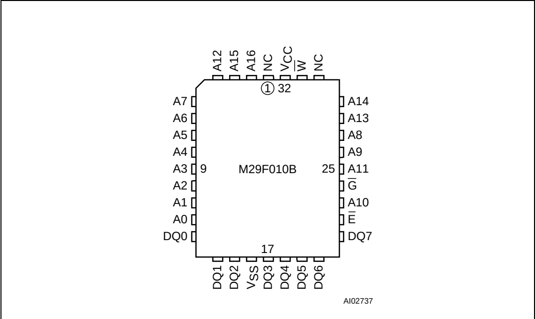
Figure 2. PLCC connections
