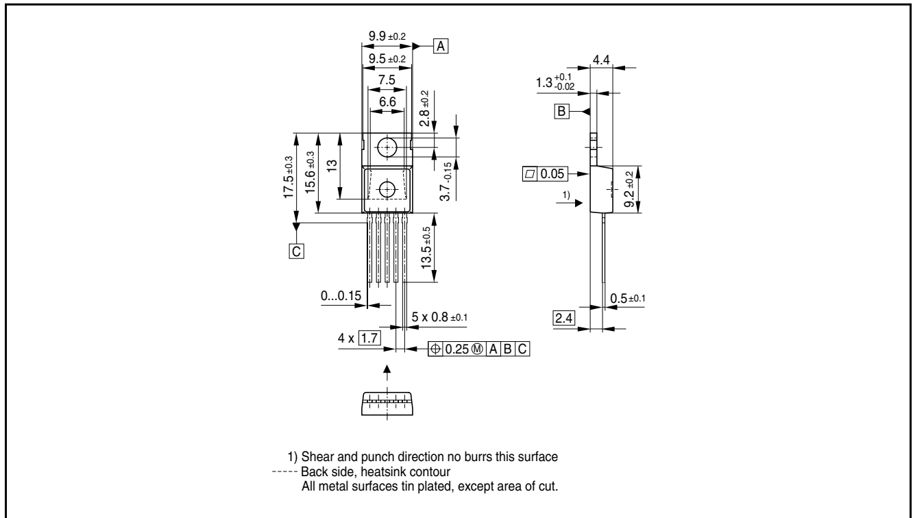
Figure 3 PG-T0220-5-43
